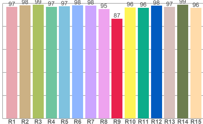
CRI: 97.4 (R1-R8)
