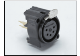
1270325 CT-Xlr-Panel-Female-5-Pin
