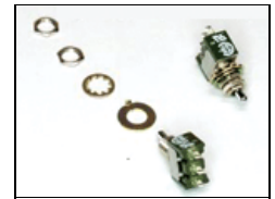
1290013 SW-Toggle-Miniature-SPDT-5A
