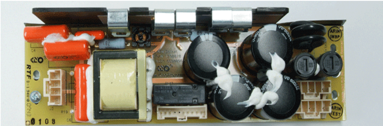
VistaBeam 600/300 Ballast Board (Part # 6800096) Top View
