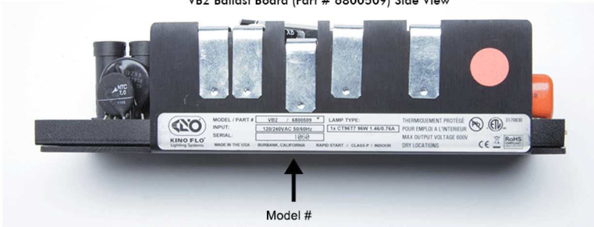
VB2 Ballast Board (Part # 6800509) Side View
