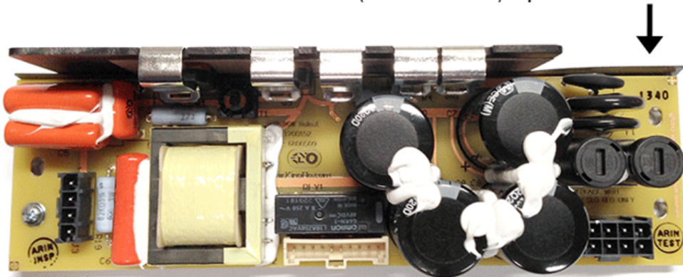
VB2 Ballast Board (Part # 6800509) Top View Date Code
