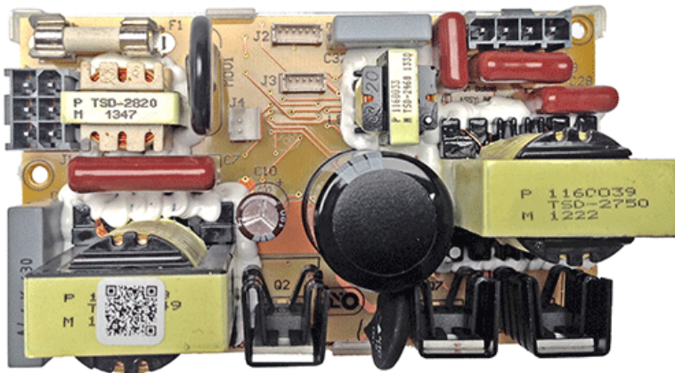
TG1 Ballast Board (Part # 6800500) Top View
