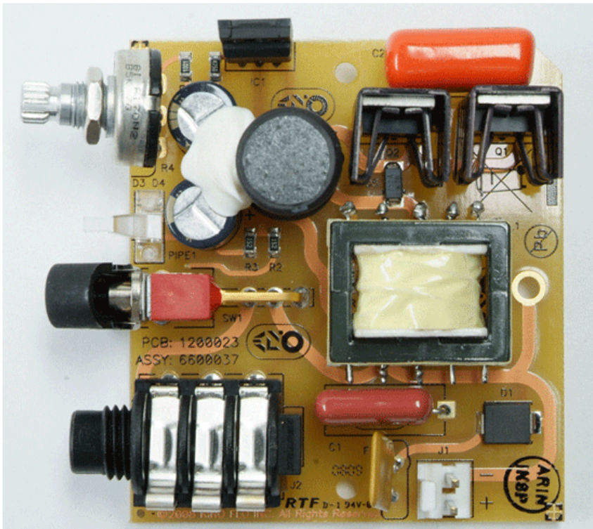
Mini-Flo 139X Ballast Board (Part # 6800037) Top View
