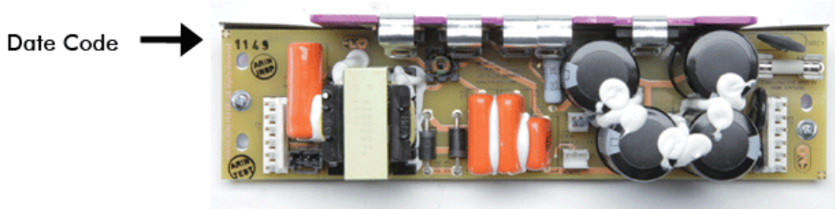
MG4R Ballast Board (Part # 6800084) Top View
