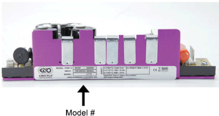
MG4R Ballast Board (Part # 6800084) Side View
