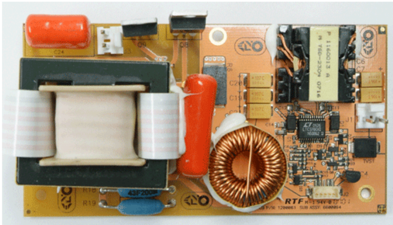
Kamio Ballast Board (Part # 6800094) Top View
