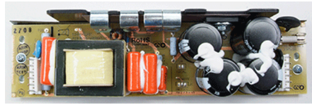
6800131 - DG4 Ballast Board
