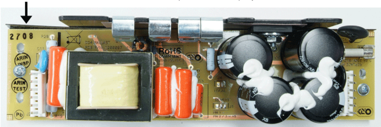
DG4 Ballast Board (Part # 6800131) Top View
