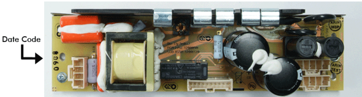
BarFly Ballast Board (Part # 6800120) Top View
