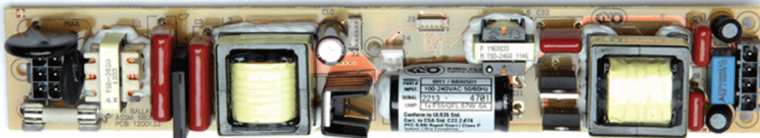
BR1 Ballast Board (Part # 6800501) Top View
