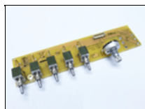
6800193 Imara S10/S100 Switch Control Board.
