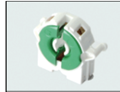
1380016 Lampholder T12 Bi-pin Twist no Spring. Used in Rev H thru I. (Replace w/ same)
