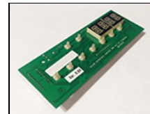
4010024 Celeb DMX Control Board 4-Jack
