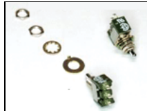
1290013 SW-Toggle-Miniature-SPDT-5A
