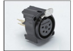
1270325 CT-Xlr-Panel-Female-5-Pin
