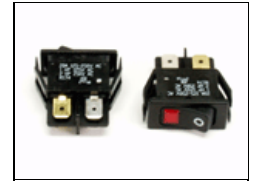
1290030 Switch-Rocker-DPST 16A-Lit-Red-250V
