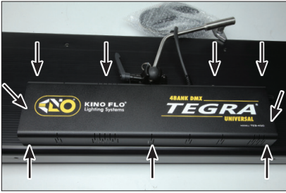
1) Remove eleven (11) cover screws.
