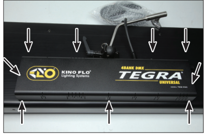
10) Replace cover with eleven (11) cover screws.
